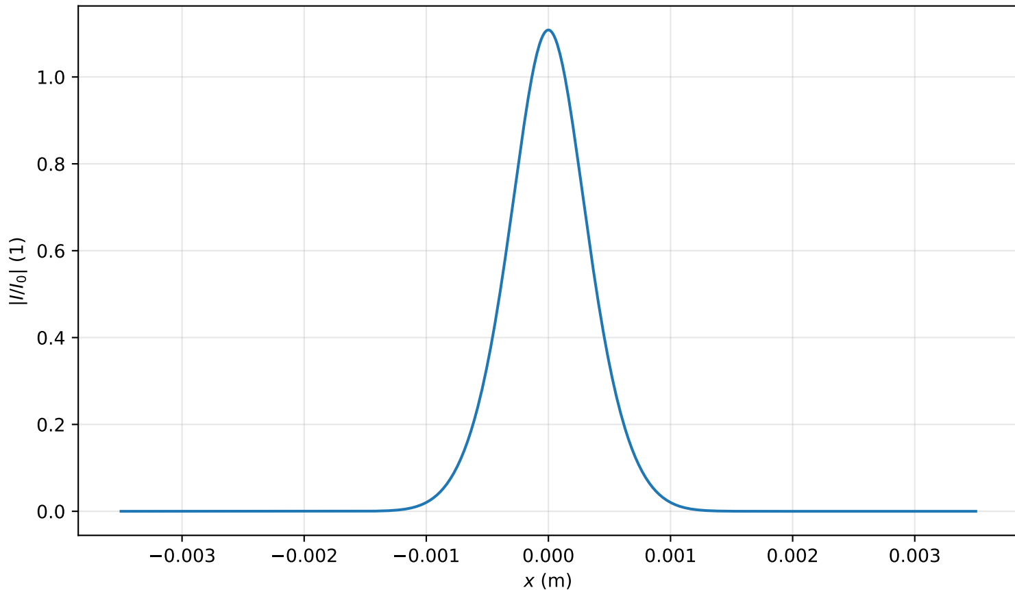
Intensity profile I(x, y = 0, z = 0.557m)/I_0 , P_{in}=0.7P_{cr} , artificial time
